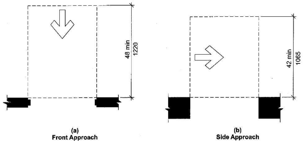
FIGURE 404.2.3.4 MANEUVERING CLEARANCE AT DOORWAYS WITHOUT DOORS
