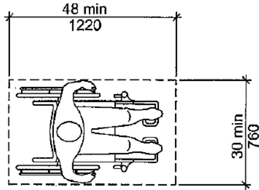
FIGURE 305.3 SIZE OF CLEAR FLOOR SPACE
