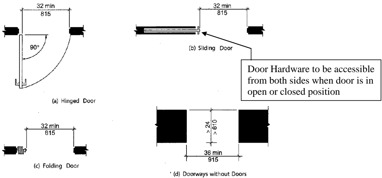
FIGURE 404.2.2 CLEAR WIDTH OF DOORWAYS
