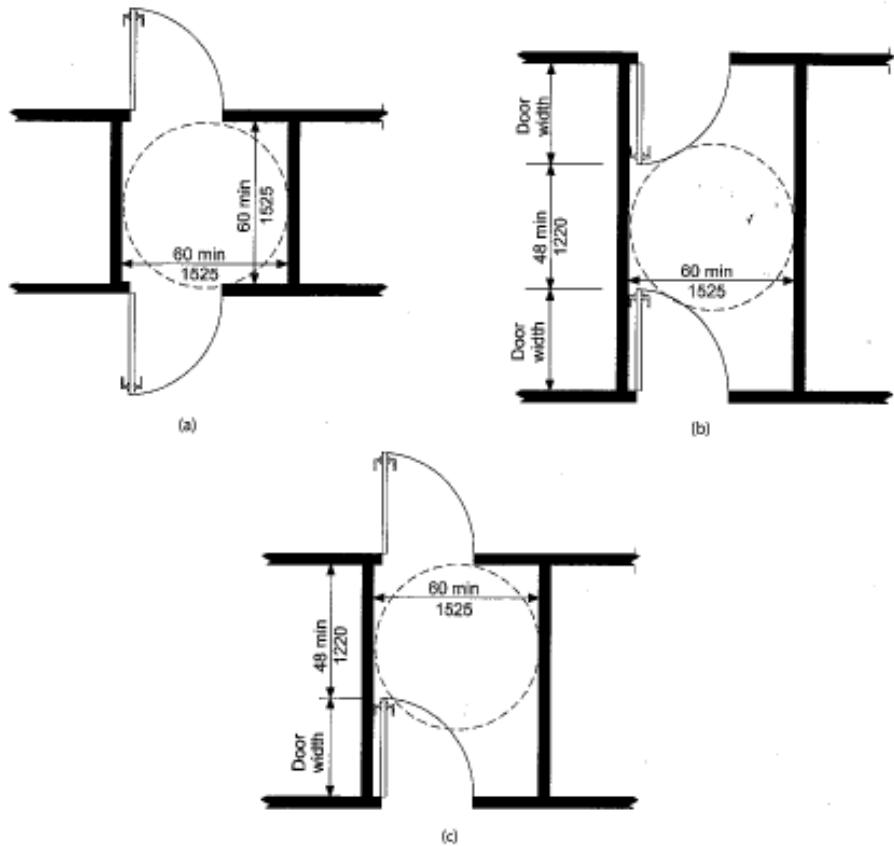
FIGURE 404.2.5 TWO DOORS IN A SERIES
