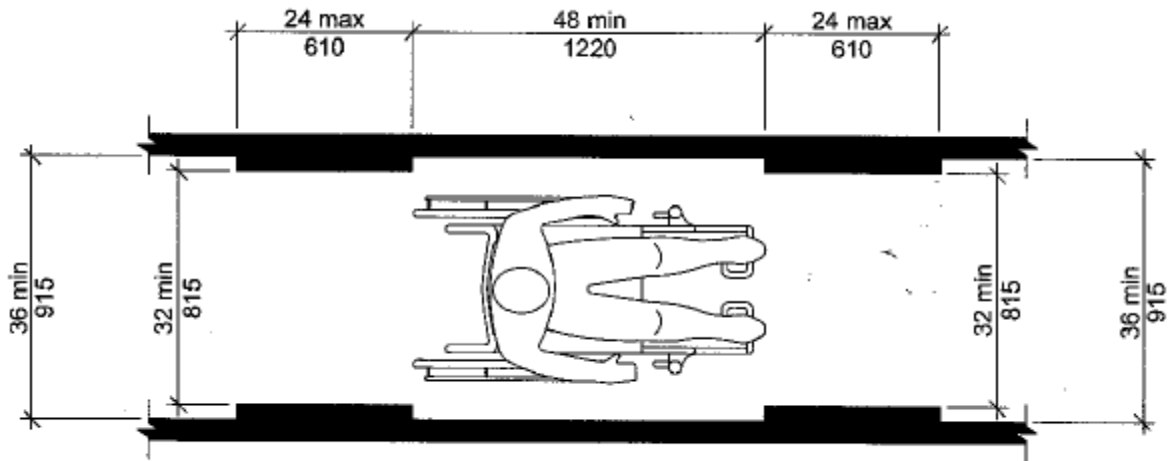
FIGURE 403.5 CLEAR WIDTH OF AN ACCESSIBLE ROUTE
