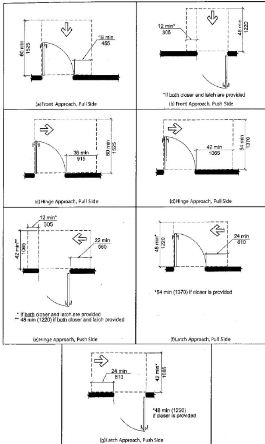
FIGURE 404.2.3.2 MANEUVERING CLEARANCE AT MANUAL SWINGING DOORS
