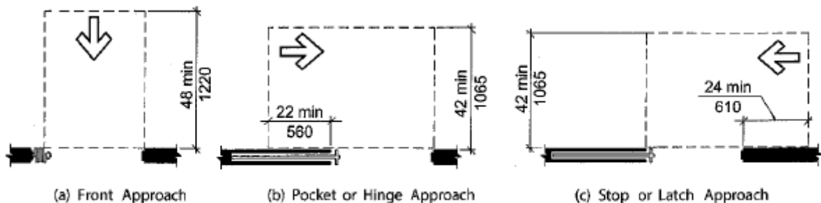
FIGURE 404.2.3.3 MANEUVERING CLEARANCE AT SLIDING AND FOLDING DOORS
