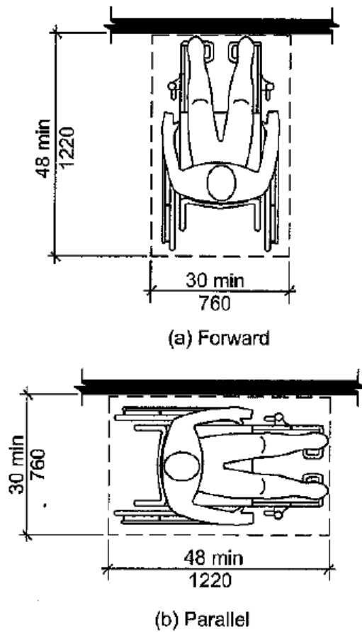
FIGURE 305.5 POSITION OF CLEAR FLOOR SPACE
