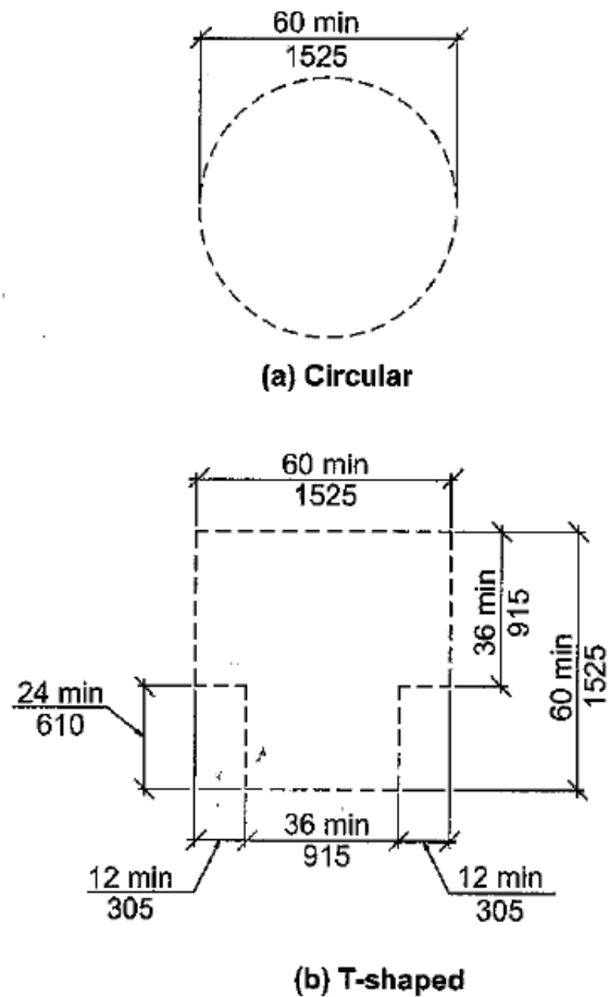
FIGURE 304.3 SIZE OF TURNING SPACE
