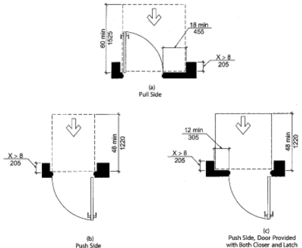
FIGURE 404.2.3.5 MANEUVERING CLEARANCE AT RECESSED DOORS
